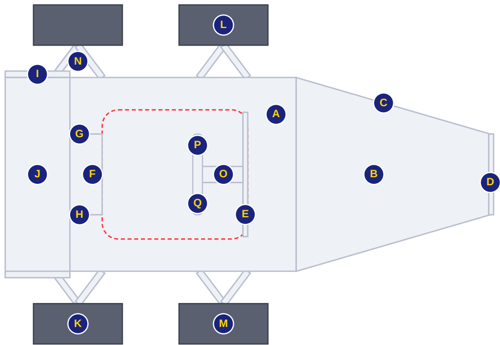
Drawn to scale from the cut sizes in this plan. Front of the car is to the right.
